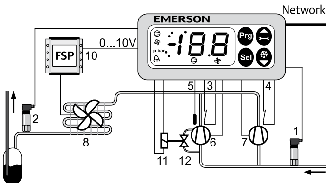
EC2-552 Condensing Unit Controller for 1 Digital Scroll and 1 single stage compressor
