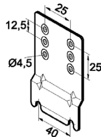
Mounting plate for units with hood Part No.: 803 801
