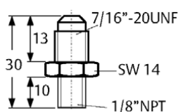
Adapter 1/8" NPT male - 7/16"-20UNF - male for compressor direct mounting Part No.: 800 316
