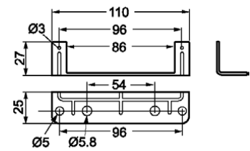
Mounting angle for TS1-Gxx / TS1-Hxx Part No.: 803 805
