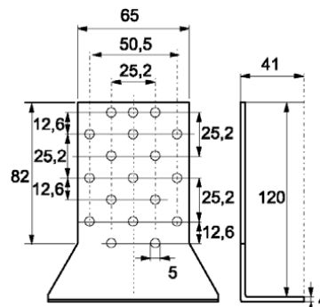
Universal mounting bracket Part No.: 803 798
