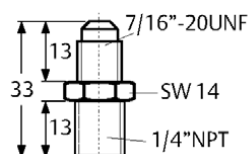
Adapter 1/4" NPT male - 7/16"-20UNF - male for compressor direct mounting Part No.: 800 315
