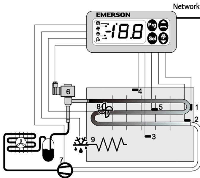
EC2-31x / -39x Case Controller (EX2, Temp/Temp)
