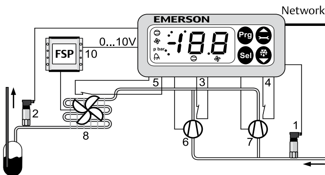
EC2-542 Condensing Unit Controller with fan speed control
