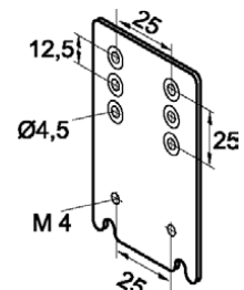
Extension bracket Part No.: 803 800
