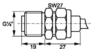
Capillary Tube Gland, Brass for Bulb Style A / C Part No.: 803 807
